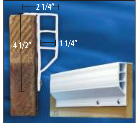
"P" Profile
